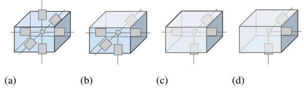
Fig. 6. Components extraction strategy for cuboid: 6(a) inside the substrate, 6(b) in the face, 6(c) in the edge, 6(d) in the vertex.
