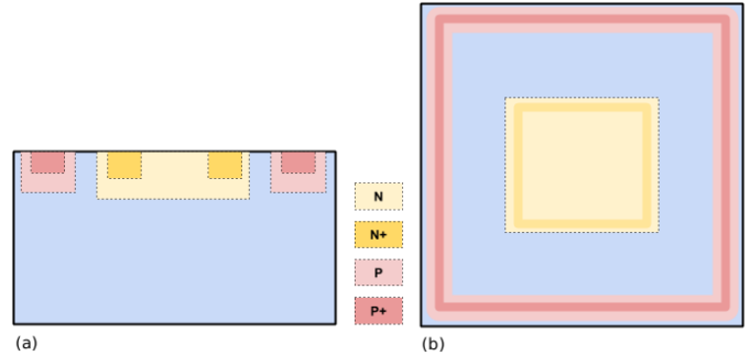
Fig. 1. Simple diode layout: (a) diode cross section view, (b) top side view.
