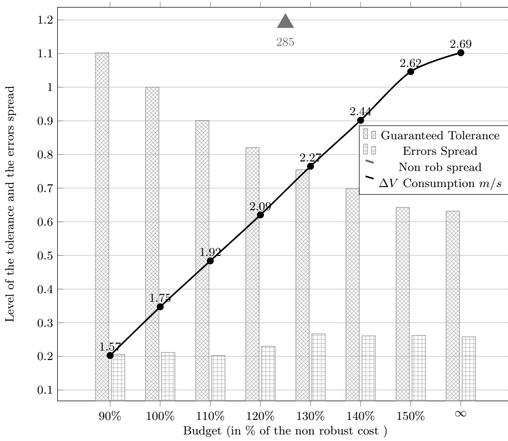
Fig. 16: Mission PROBA 3 : Rendezvous under impulses execution errors
