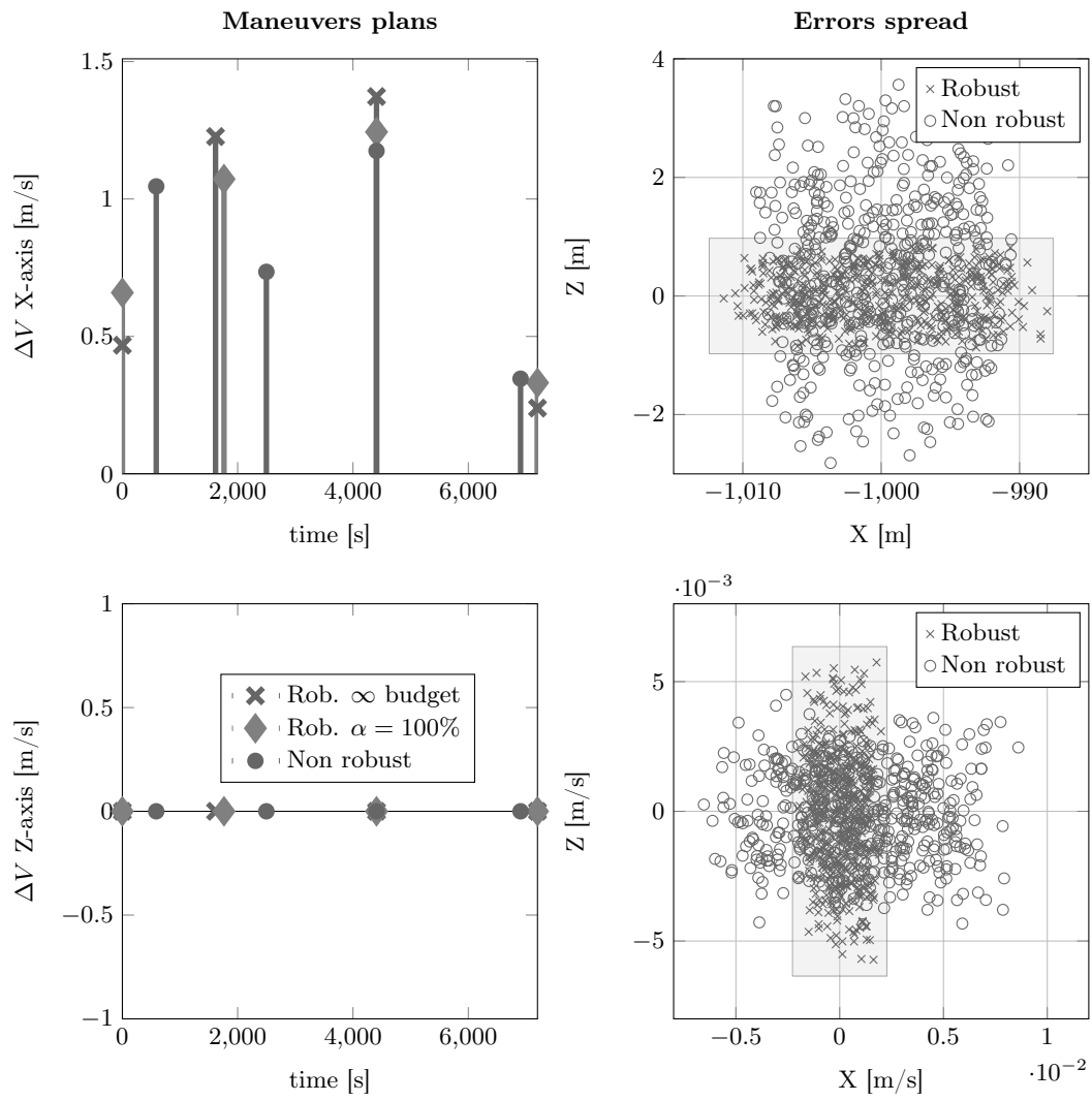
Fig. 8: Mission ATV 2: Rendezvous under uncertain impulses time
