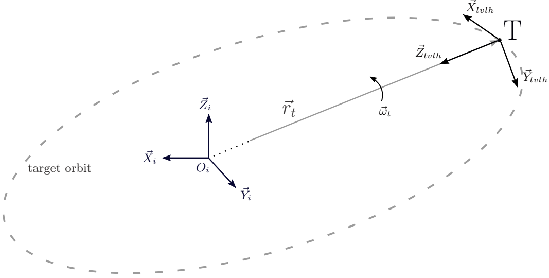
Fig. 1: Illustration of the LVLH frame
