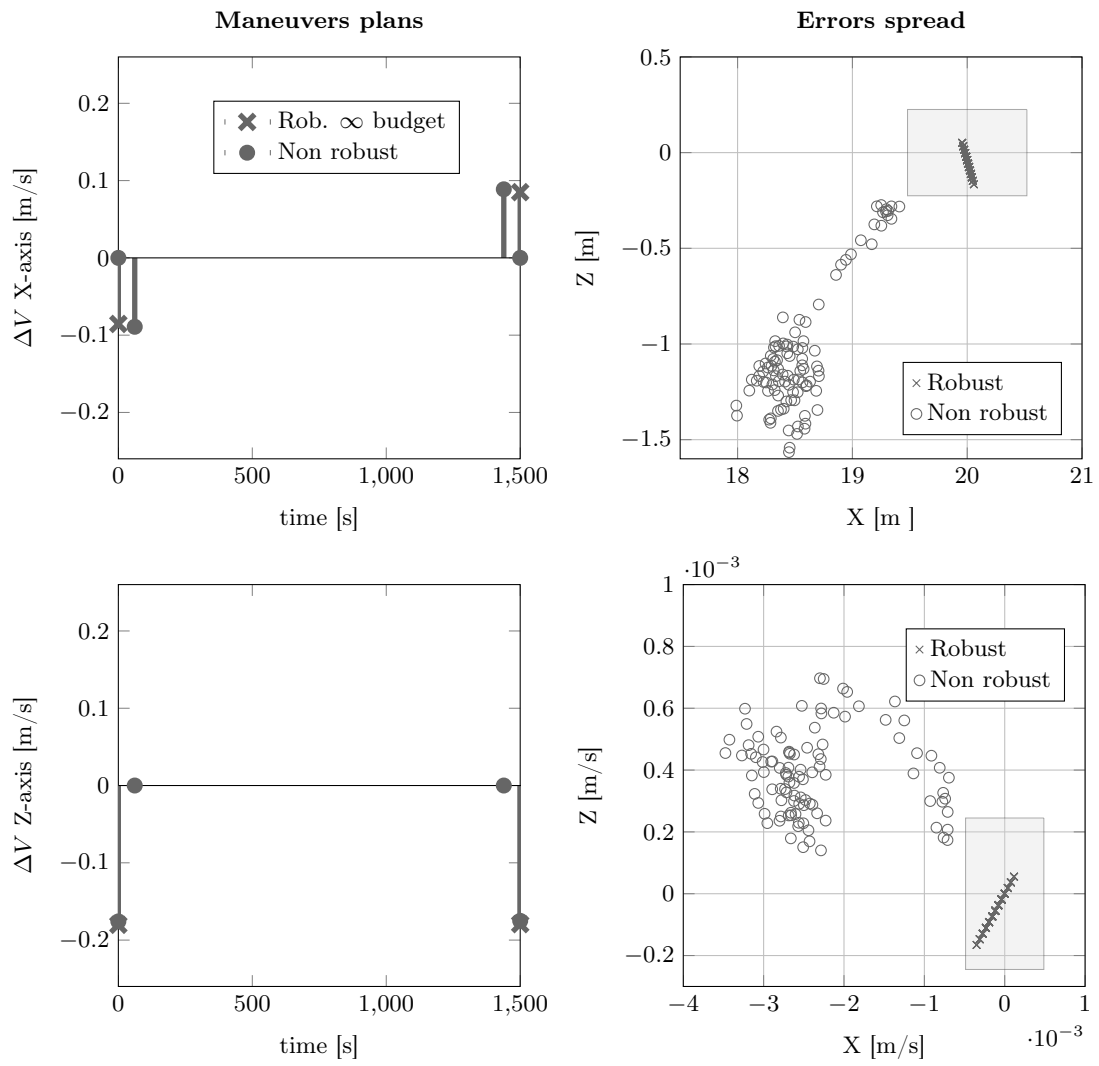
Fig. 18: Mission PRISMA : Rendezvous under uncertain impulsion times
