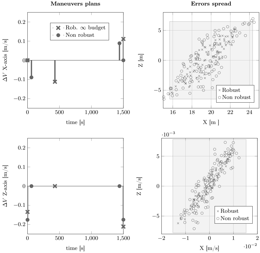
Fig. 19: Mission PRISMA : Rendezvous under impulsion execution errors
