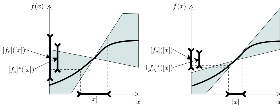
Fig. 21: Interpretation of the centred inclusion function
