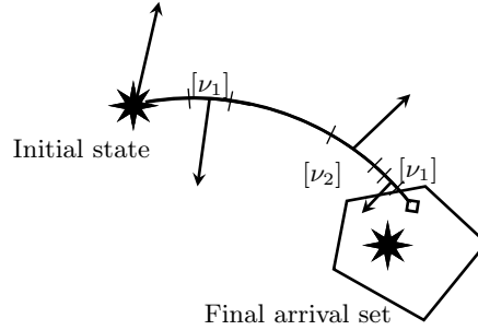
Fig. 4: polytopic rendezvous condition under impulse firing time uncertainties
