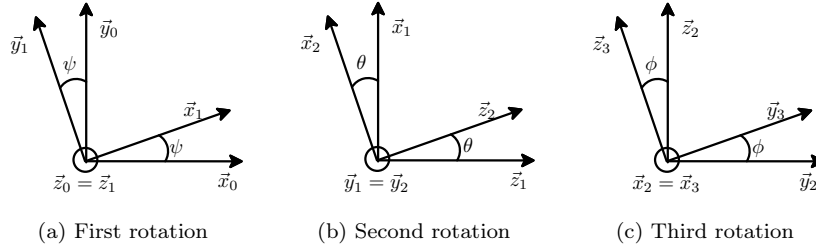
Fig. 6: Cardan angles: rotation from frame (\vec{x}_0, \vec{y}_0, \vec{z}_0) to (\vec{x}_3, \vec{y}_3, \vec{z}_3)
