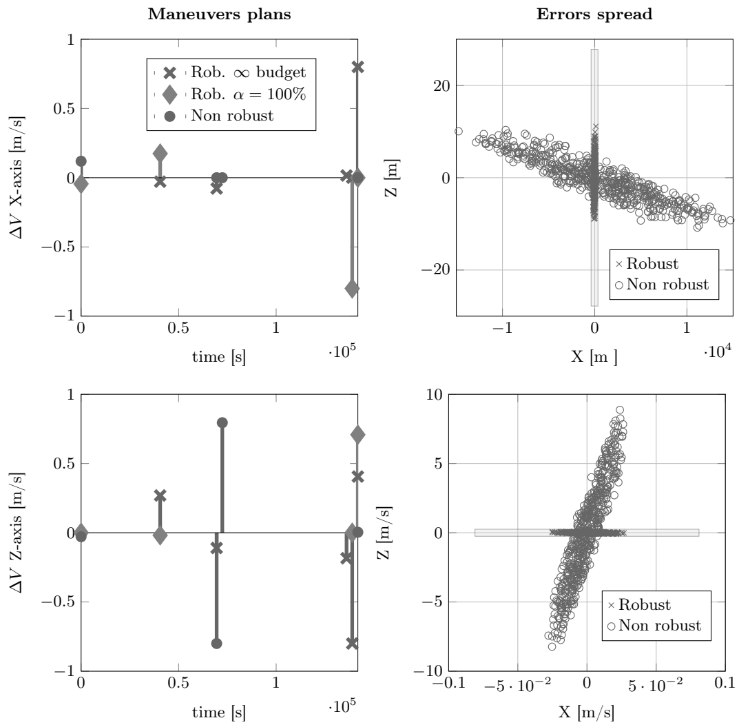
Fig. 15: Mission PROBA 3 : Rendezvous under impulses execution errors
