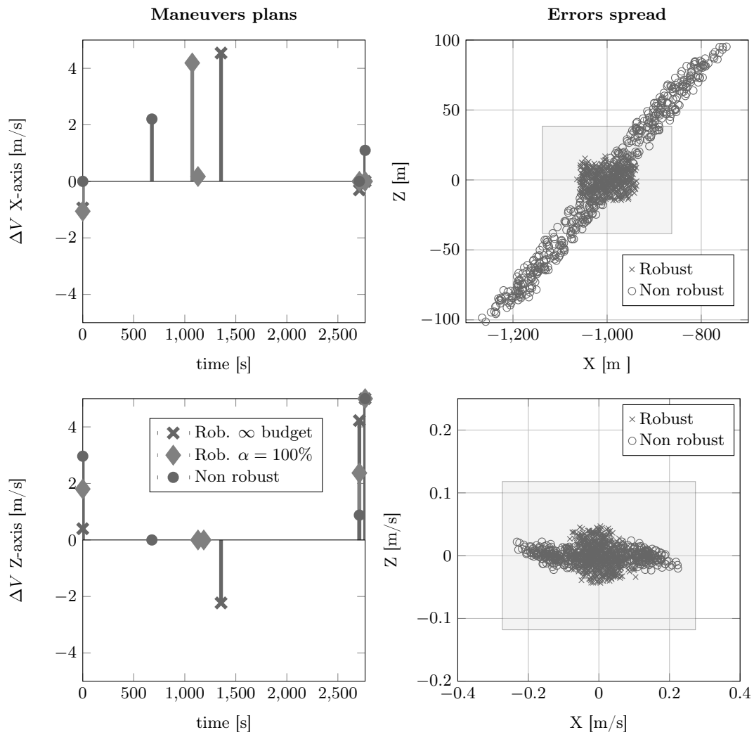
Fig. 13: Mission ATV 1: Rendezvous under impulses execution errors
