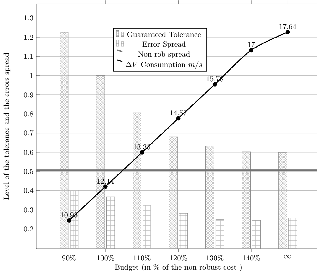
Fig. 14: Mission ATV 1: Rendezvous under impulses execution errors
