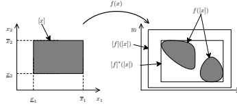
Fig. 20: Image of a box by a vector function \mathbf{f} and two of its inclusion functions [\mathbf{f}] and [\mathbf{f}]^* ; [\mathbf{f}]^* is minimal
