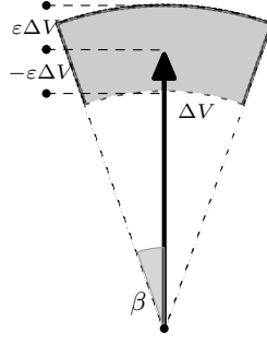
Fig. 5: Impulse execution errors description
