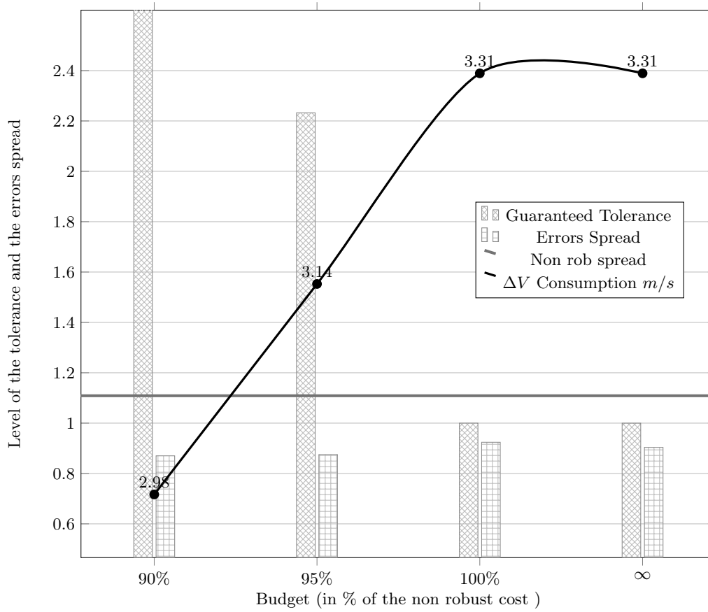
Fig. 9: Mission ATV 2: Rendezvous under uncertain impulses time
