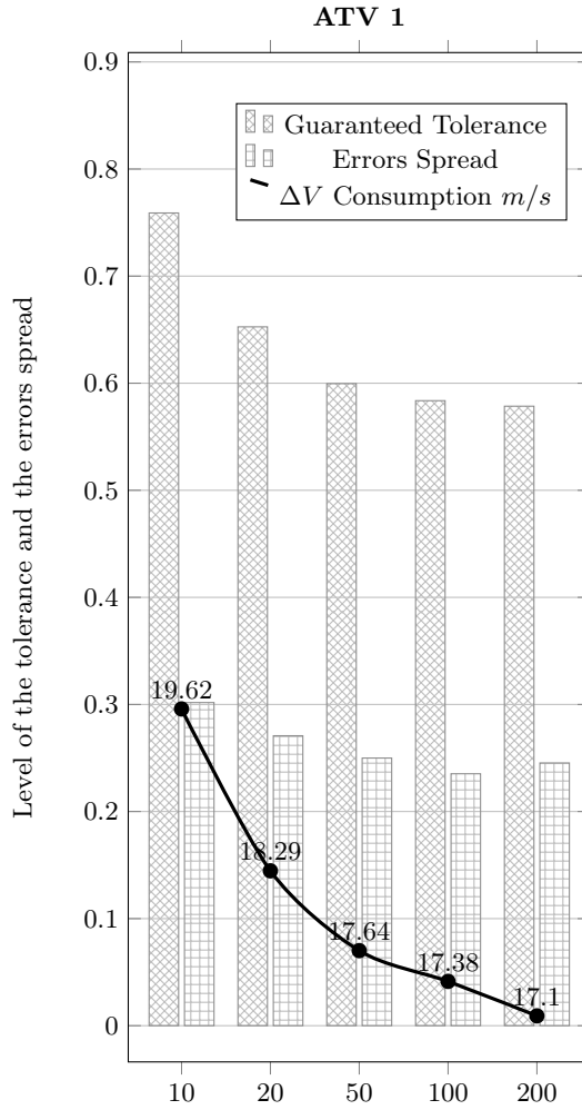
Fig. 17: Rendezvous under impulses execution errors with varying number of impulses N
