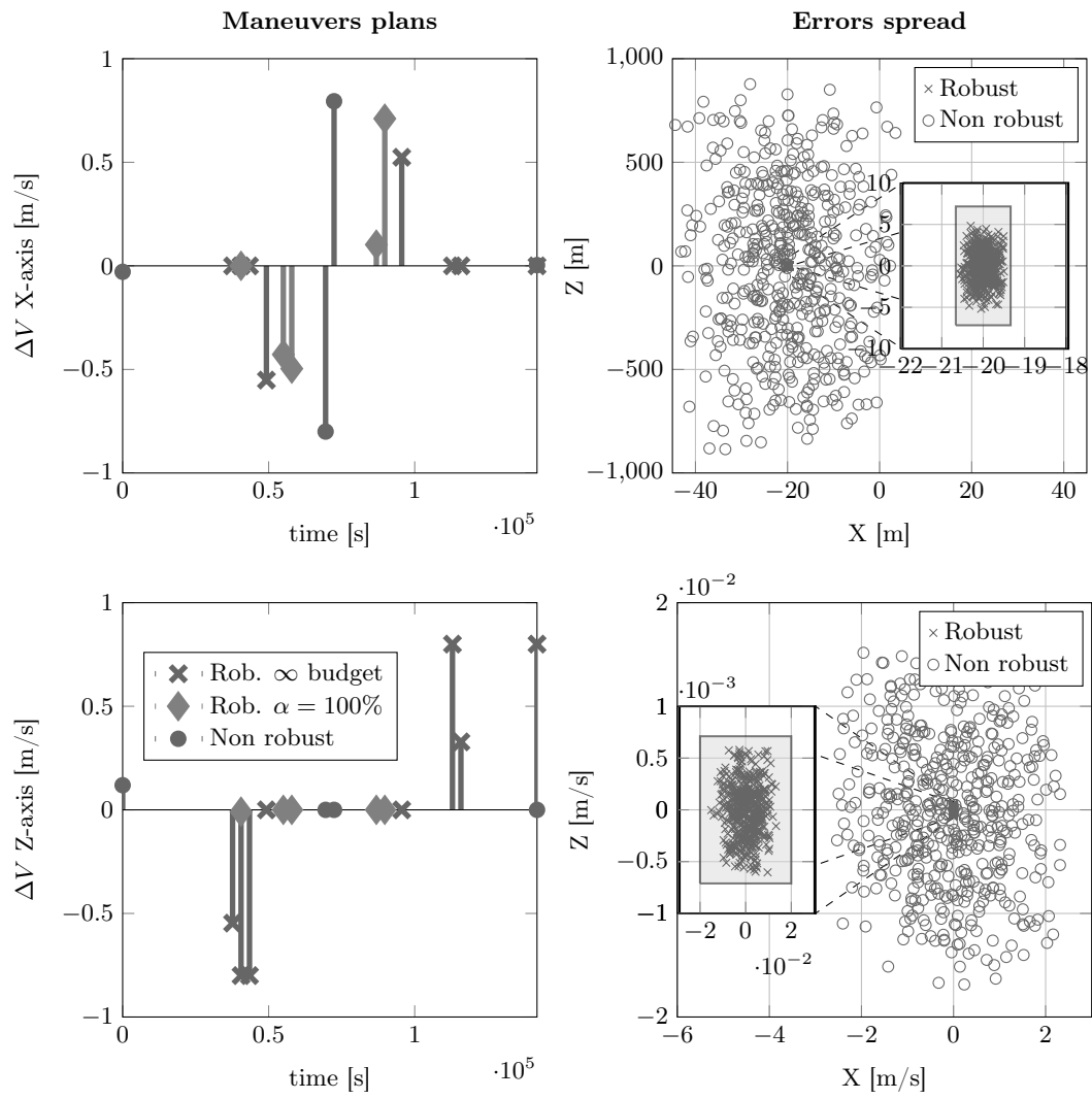
Fig. 10: Mission PROBA 3 : Rendezvous under uncertain impulses time
