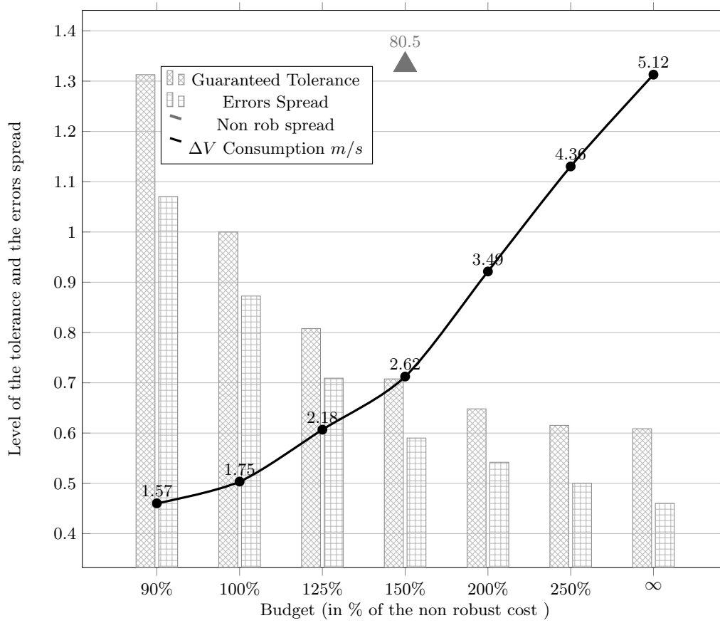
Fig. 11: Mission PROBA 3 : Rendezvous under uncertain impulses time
