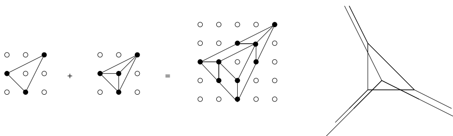
FIGURE 13. Three intersection points and D(\mathcal{W}_1, \mathcal{W}_2) = 3 .
