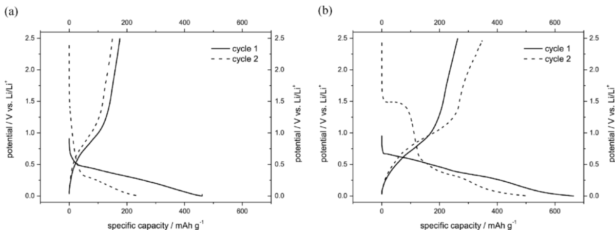
Fig. 7. Voltage profile of electrodes containing (a) \text{Li}_2\text{CuSn}_2 and (b) \text{Li}_2\text{AgSn}_2 as the active materials in the voltage range between 0 and 2.5 V vs. \text{Li}/\text{Li}^+ . The tests were carried out using a C-rate of C/5.
