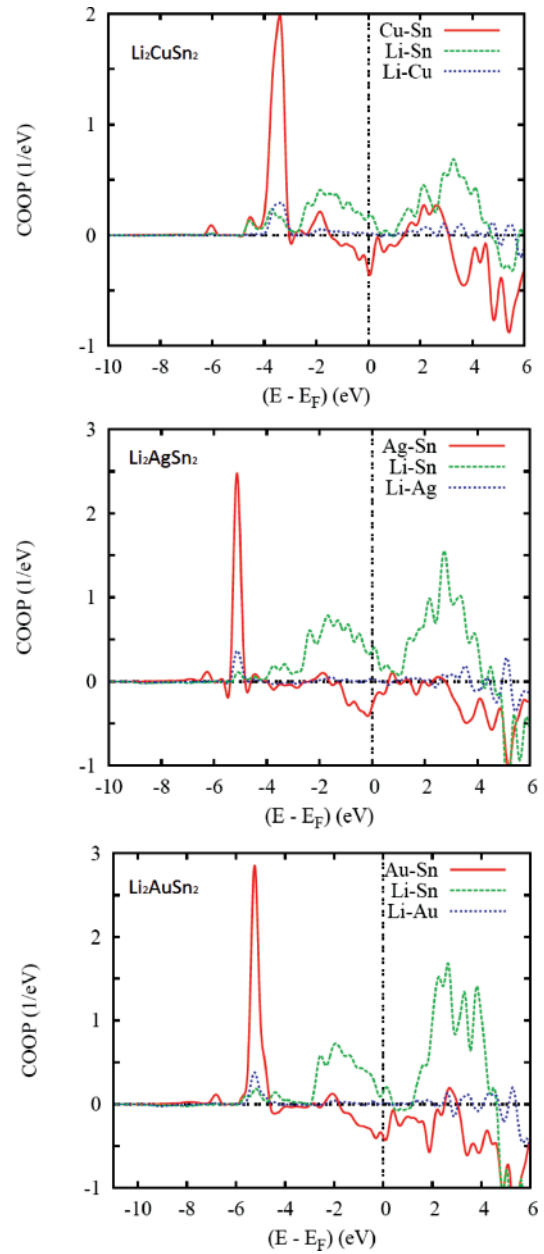
Fig. 3 (color online). Chemical bonding for pair interactions in the stannides \text{Li}_2T\text{Sn}_2 .
