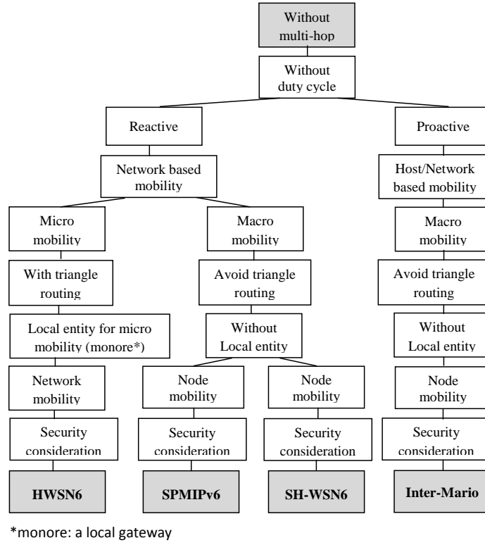
Figure 7: Classification of mobility support protocols for 6LoWPAN Networks without multi-hop consideration
