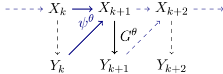
Figure 1: Graphical representation of the observation-driven model.
