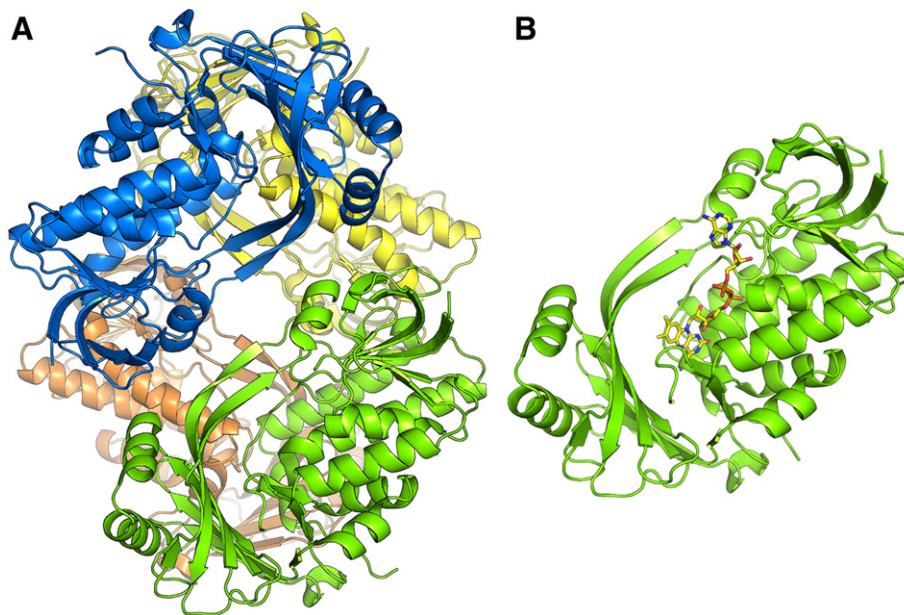
Fig. 6. Structure of the Ubil monoxygenase from Escherichia coli . A. Crystal structure of the C-terminal truncated form of E. coli C5-hydroxylase Ubil involved in Q_8 biosynthesis, 2.0 Å resolution (PDB ID: 4 K22) [32]. B. Proposed molecular docking model of Ubil with FAD. The flavin cofactor is shown as yellow sticks.
