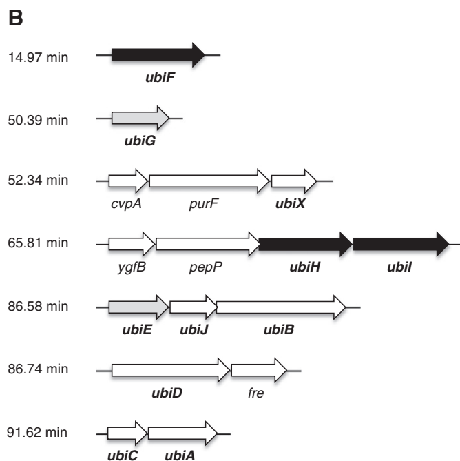
Fig. 2. Genetic organization and location of ubi genes on the Escherichia coli chromosome. A. Location of the eleven ubi genes on the 100 min map of the E. coli chromosome. B. Genetic organization of the ubi genes in E. coli . The location of each gene (or the first gene of the operon) is indicated on the left. The genes required for ubiquinone biosynthesis are indicated in bold. Genes encoding monooxygenases are symbolized by black arrows and genes encoding methyltransferases are symbolized by gray arrows.
