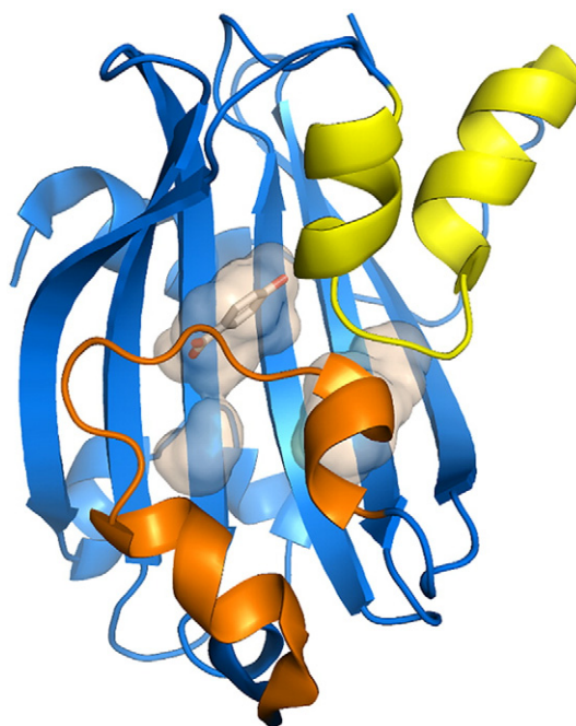
Fig. 3. Structure of the chorismate lyase UbiC from Escherichia coli . Crystal structure of the chorismate lyase UbiC from E. coli in complex with the 4-hydroxybenzoate, 1.0 Å resolution (PDB ID: 1TT8) [37]. The core of the protein fold is a 6-stranded antiparallel β-sheet, with two helix–turn–helix loops colored in yellow and orange. The two internal cavities are colored in gray. The 4-HB product is located in one of these cavities, behind the two flaps in a hydrophobic pocket.
