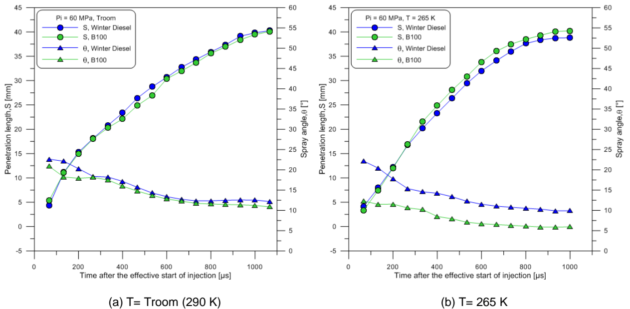
Figure 11. Penetration length and spray angle - P_i = 60 MPa, \rho_a = 20.1 kg/m 3 .
