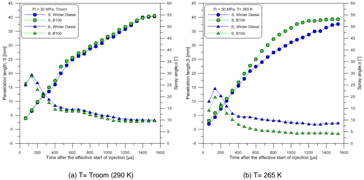
Figure 10. Penetration length and spray angle - P_i = 30 MPa, \rho_a = 20.1 kg/m 3 .
