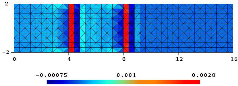
Fig. 5. Illustration of the total height L^\infty -error field for the 800 cells mesh when a \mathbb{P}_2 polynomial reconstruction is used with stencils that are not topologically constrained.
