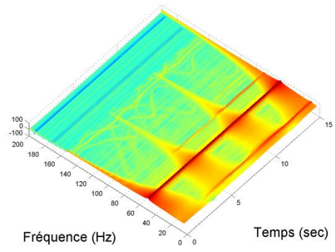
(c) Scalogramme
