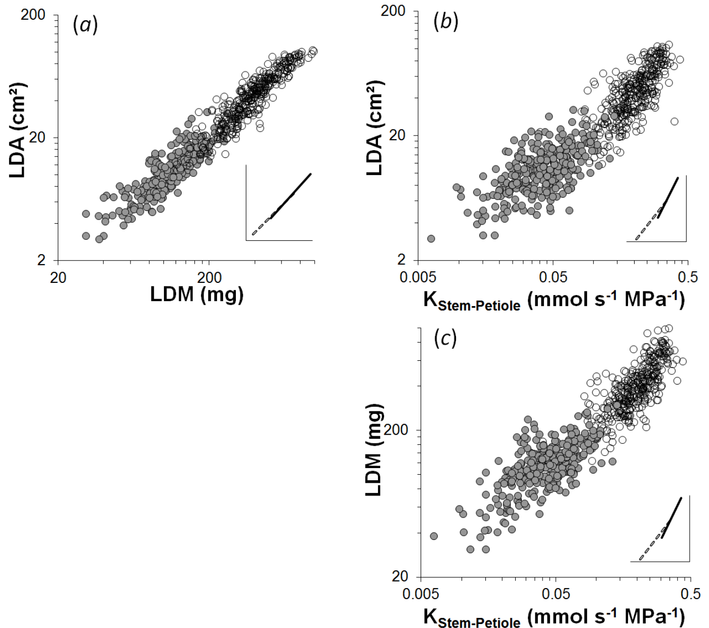
Figure 3: Covariation between leaf traits (a), and between each leaf trait and the stem-to-petiole continuum maximal xylem conductance, K_{\text{Stem-Petiole}} (b-c) in Log 10 axes. Bivariate line fitting with standardized major axis method (SMA) for log 10 –log 10 relationships between leaf dry area (LDA) and leaf dry mass (LDM) (a), leaf dry area (LDA) and K_{\text{Stem-Petiole}} (b), and leaf dry mass (LDM) and K_{\text{Stem-Petiole}} (c). Data are for 17 apple genotypes including the two parent cultivars, ‘Starkrimson’ and ‘Granny Smith’, and 15 of their progenies, cultivated in two water regimes, well-watered (WW, open circle) and water-stressed (WS, grey circle). Each symbol represents one leaf. For each relationship, fitting lines are figured in inset. Fitting lines parameters are detailed in Table 1.
