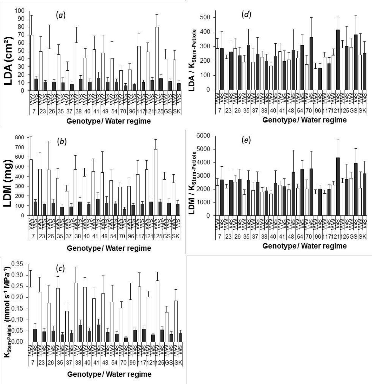
Figure 1: Variations of individual leaf traits across apple genotypes and water regimes, leaf dry area (LDA) (a), leaf dry mass (LDM) (b), K_{\text{Stem-Petiole}} (c), and the two ratios LDA/ K_{\text{Stem-Petiole}} (d) and LDM/ K_{\text{Stem-Petiole}} (e). Data (mean+SD) are for 17 apple genotypes including the two parent cultivars, ‘Starkrimson’ (SK) and ‘Granny Smith’ (GS), and 15 of their progenies identified by their number, in two water regimes, well-watered (WW; white bars) and water-stressed (WS; black bars). For LDA, LDM and K_{\text{Stem-Petiole}} , each genotype shows a significant difference (t-test, P < 0.01 ; data not shown) between WW and WS values. For LDA/ K_{\text{Stem-Petiole}} and LDM/ K_{\text{Stem-Petiole}} WW and WS values are similar or differed depending on the genotype (t-test, P < 0.01 ; data not shown, see text).
