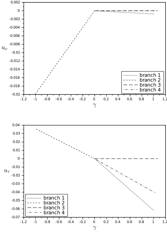
Fig. 14 Bifurcation diagrams.
