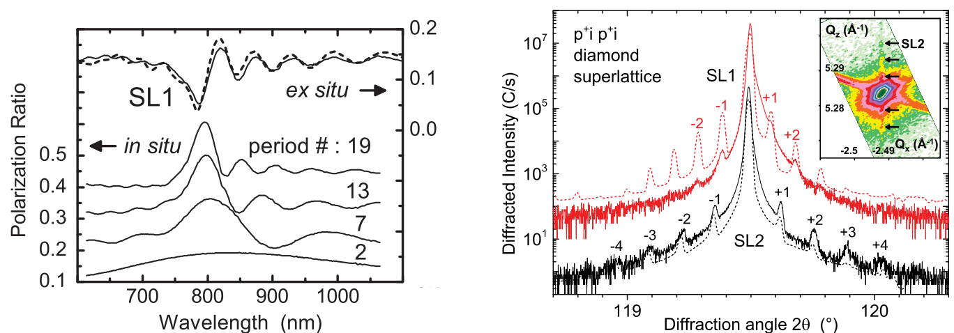
FIG. 2. Bottom, left-hand scale: polarization ratio spectra determined in situ by ellipsometry under a 71^\circ incidence during the periodic growth of p^+/i bilayers after 2, 7, 13, and 19 epitaxial growth cycles for sample SL1. Top, right-hand scale: experimental (solid) and simulated (dashed) polarization ratio spectra of sample SL1 as measured ex situ at room temperature (angle of incidence: 75^\circ ).
