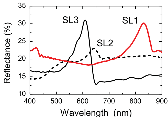
FIG. 3. Reflectance spectra of diamond doping superlattices SL1, SL2, and SL3 measured at room temperature under an angle of incidence of 12 \pm 3^\circ .
