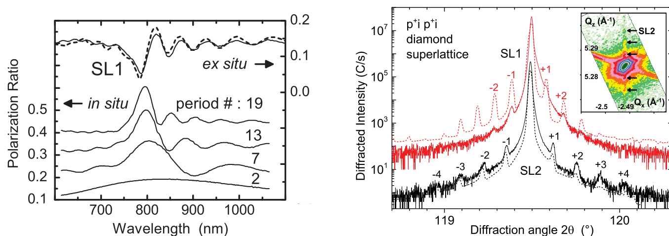
FIG. 2. Bottom, left-hand scale: polarization ratio spectra determined in situ by ellipsometry under a 71^\circ incidence during the periodic growth of p + / i bilayers after 2, 7, 13, and 19 epitaxial growth cycles for sample SL1. Top, right-hand scale: experimental (solid) and simulated (dashed) polarization ratio spectra of sample SL1 as measured ex situ at room temperature (angle of incidence: 75^\circ ).
