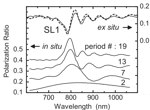
FIG. 2. Bottom, left-hand scale: polarization ratio spectra determined in situ by ellipsometry under a 71^\circ incidence during the periodic growth of p + / i bilayers after 2, 7, 13, and 19 epitaxial growth cycles for sample SL1. Top, right-hand scale: experimental (solid) and simulated (dashed) polarization ratio spectra of sample SL1 as measured ex situ at room temperature (angle of incidence: 75^\circ ).
