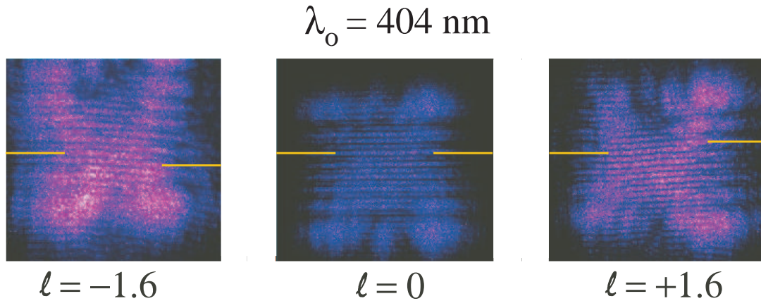
Figure 5. Interference pattern of a blue twisted beam. The measured fractional topological charge are \ell = -1.6 , \ell = 0 and \ell = +1.6 . The yellow lines indicate the constructive interference on each end of the pattern.
