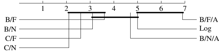
Fig. 3. Post-hoc test results on algorithms. Thick lines links non-significantly different algorithms.
