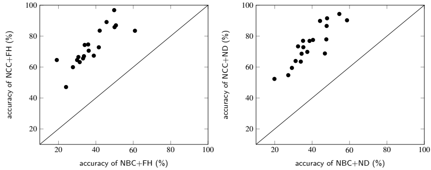
Fig. 4. Non-discounted accuracy of the NBC vs NCC methods for both decompositions on indeterminate instances
