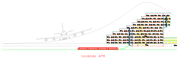
Fig. 6. Parking lots located under the hump of the runway
