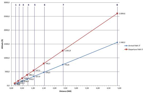
Fig. 12. TMA routes (vertical view)
