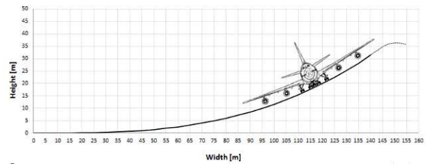
Fig. 1. Runway profile
