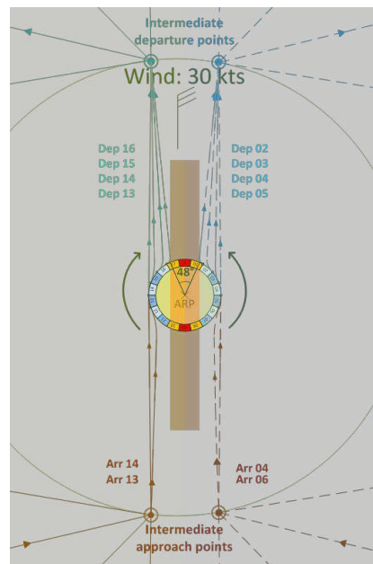
Fig. 13. Operations in strong wind conditions
