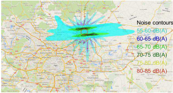
Fig. 21. Noise contours comparison between The Endless Runway and Paris Charles de Gaulle airports
