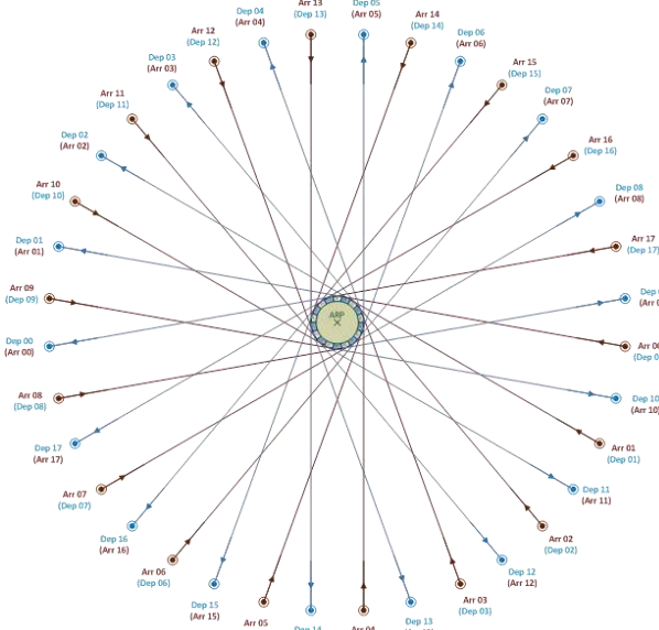
Fig. 11. TMA layout (top view)
