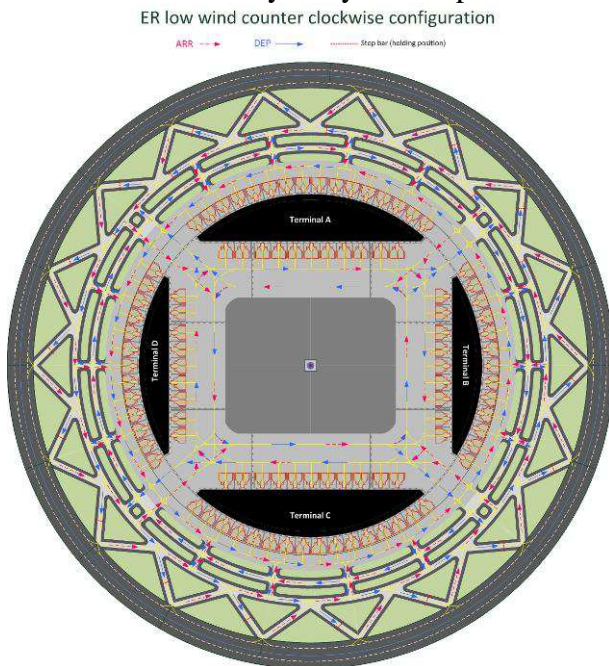
Fig. 7. Endless Runway runway and taxiways
