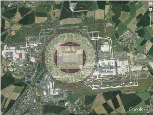
Fig. 9. Impression of an Endless Runway airport footprint overlaid at Paris CdG
