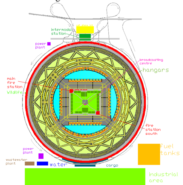
Fig. 5. The Endless Runway hub airport layout
