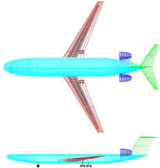
Fig. 3. Plan views of ERAC
