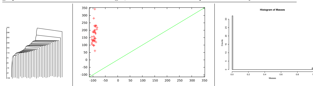
Figure 13 Disconnectivity tree, persistence diagram, and histogram of masses for the T-RRT run started near the local minimum of 6 . The vertex weighted transition graph contains 33 vertices and 60 edges; it has 1 connected component and 28 cycles.
