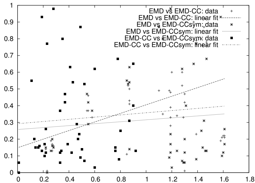
Figure 22 Correlation between the transport costs delivered by EMD and EMD (both ways), on runs of T-RRT started near the 10 lowest local minima, with uniform masses (see text for details) The Pearson coefficients are respectively equal to 0.44, 0.09 and 0.06 for the three pairs.
