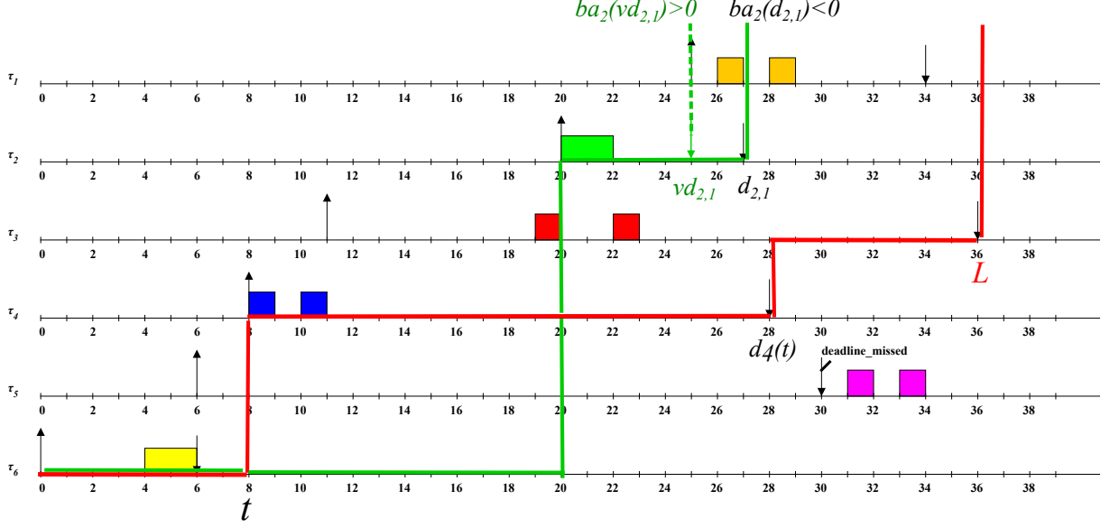
Figure 13: Interdependency between virtual deadlines
