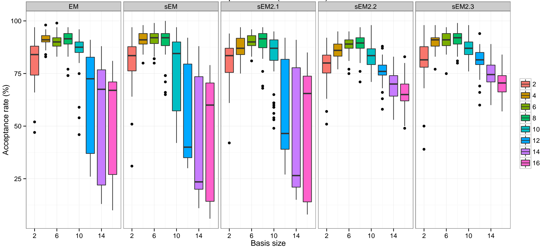
Acceptance rate (coefficients)
