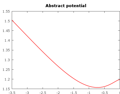
FIGURE 13. Plot of the potential function \mathcal{U} over [\phi_w, 0] for \alpha = 0 .
