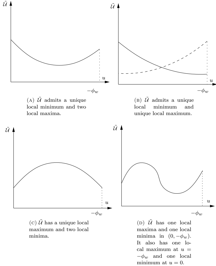
FIGURE 5. Plots of all possible behavior of the function u \in [0, -\phi_w] \mapsto \tilde{\mathcal{U}}(u) . The function studied in the scope of theorem 3.2 corresponds to the dashed line of Figure (B).
