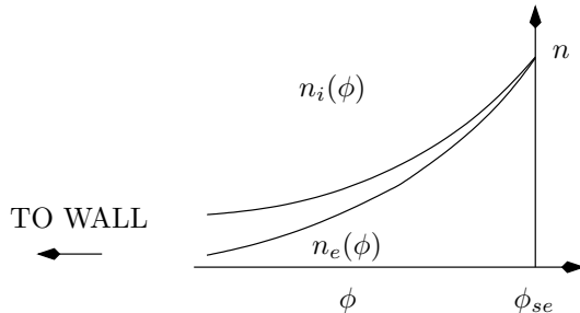
FIGURE 1. Schematic variations of the ion and electron densities with respect to some normalized potential \phi \leq 0 decreasing toward the wall. Here the plasma is supposed to be neutral at the sheath-edge x_{se} .
