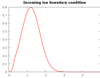
FIGURE 6. Plot of the incoming ion boundary condition for positive velocities with Z = \frac{3}{2} .
