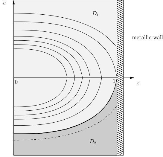
FIGURE 3. Schematic characteristic electron trajectories associated with a decreasing potential \phi . The dashed line corresponds to a characteristic curve which originates at the wall with a negative velocity. Because of the boundary condition at the wall, particles following this curve were originally at x = 0 with a positive velocity.
