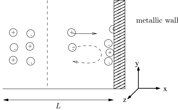
FIGURE 2. Schematic illustration. Ions and electrons are going toward the wall, some electrons reaching the wall are re-emitted with a probability \alpha \in [0, 1] while ions are totally absorbed.
