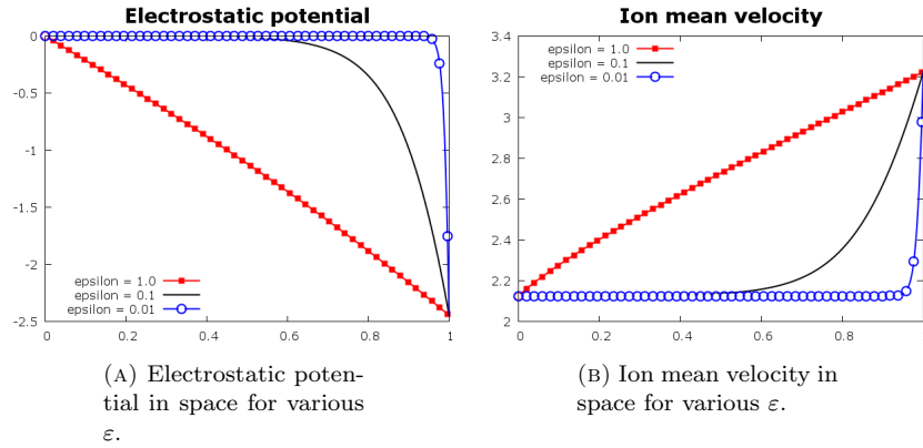
FIGURE 11. Electrostatic potential and ion mean velocity in the domain [0, 1] for various values of \varepsilon .
