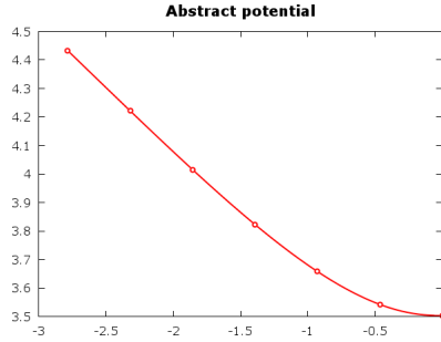
FIGURE 7. Plot of the potential function \mathcal{U} over [\phi_w, 0] for \alpha = 0 .
