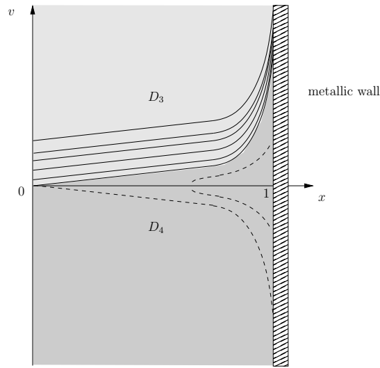
FIGURE 4. Schematic characteristic ions trajectories associated with a decreasing potential \phi . Here the dashed lines correspond to characteristic curves originating from the wall with negative velocities, and they span the darker gray region D_4 . Because of the boundary condition at the wall, no particles travel on these curves and hence f_i vanishes outside D_3 (lighter gray).
