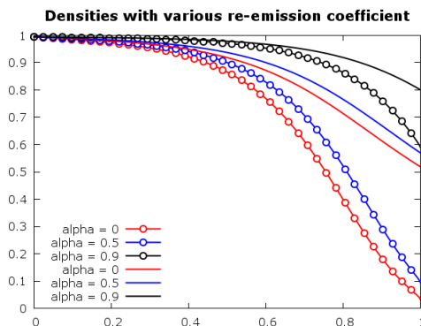
FIGURE 12. Ion and electron densities for \varepsilon = 0.1 and \alpha \in \{0, 0.5, 0.9\} . Pointed lines correspond to electron densities and thick lines to ion densities.
