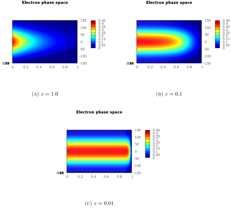
FIGURE 9. Electron distribution functions in the phase space for various \varepsilon . Plot (a),(b) and (c) are represented in the phase space [0, 1] \times [-150, 150] .
