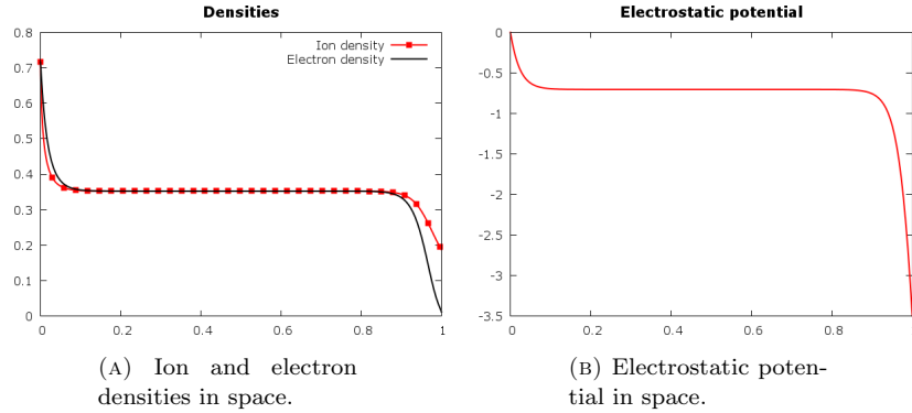
FIGURE 15. Macroscopic densities and electrostatic potential in space. Plot (a),(b) are represented in the space [0, 1] .
