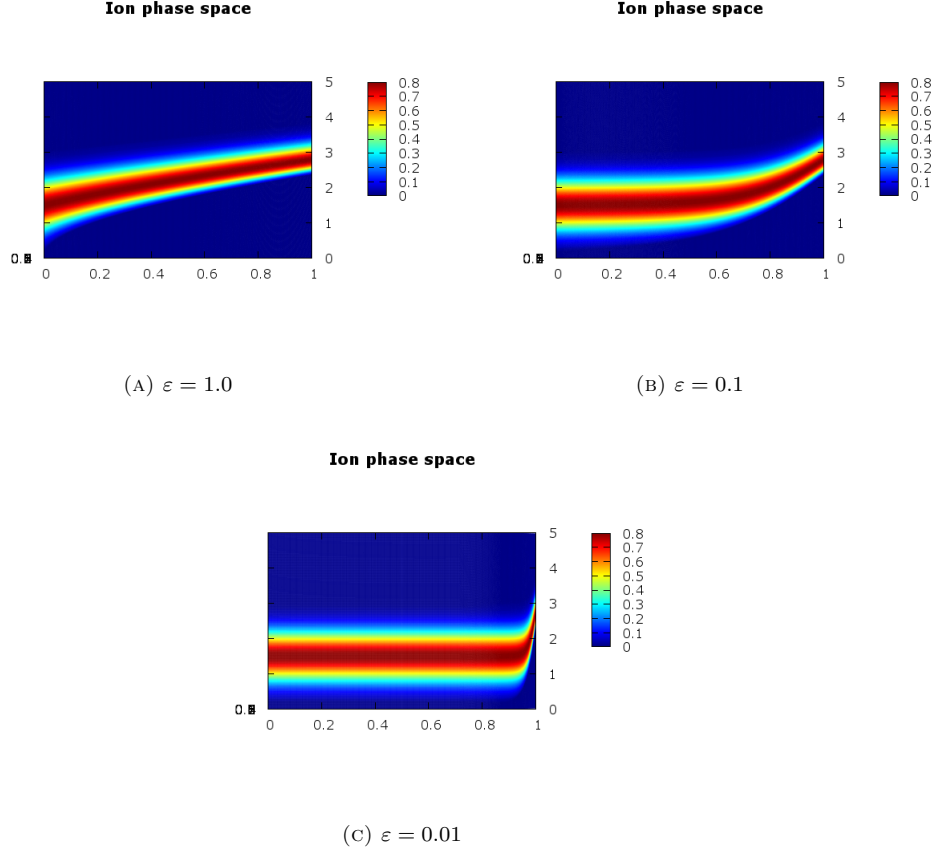
FIGURE 8. Ion distribution functions in the phase space for various \varepsilon . Plot (a),(b) and (c) are represented in the phase space [0, 1] \times [0, 5] .
