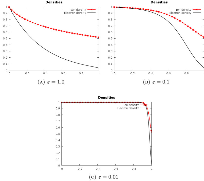
FIGURE 10. Ion and electron densities in space for various \varepsilon . Plot (a),(b),(c) are represented in the space [0, 1] .
