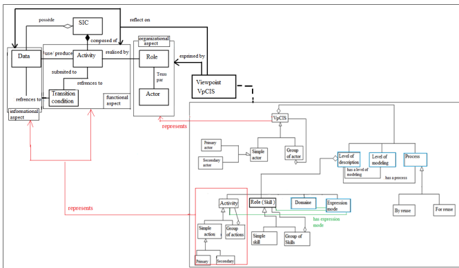
Figure 2. CIS meta-model integrating VpCIS meta-model
