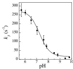
Figure 4. pH-dependence of the rate constant k_3 for the reaction of the wt SOR from D. baarsii (100 μM) with O 2 •- (8-12 μM), generated by pulse radiolysis in the presence of 10 mM formate and 2 mM buffer. Tungsten lamp with a 345 nm cut-off filter. The titration curve fitted the equation expected from a single protonation process, k_3 = (k_{3max} + k_{3min} \times 10^{(pH-pK_a)}) / (1 + 10^{(pH-pK_a)}) . A pK a value of 7.2 ± 0.1 was determined.
