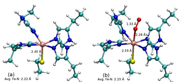
Figure 7. Optimized structures for reduced SOR (a) and reduced SOR with superoxide substrate (b), geometries optimized using the B3LYP/double- \zeta level of theory.
