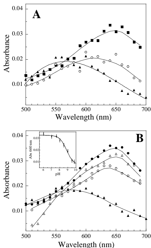
Figure 3. Absorption spectra (tungsten lamp with a 345 nm cut-off filter, 2 cm path-length cuvette) at various pH values of the P1 transient and of the final species P2 formed after the reaction of the SOR wt from D. baarsii with O_2^{\bullet-} (8 \mu M), generated by pulse radiolysis in the presence of 10 mM formate and 2 mM buffer. A. Spectra of P1 at pH 6.0 and 5 ms after the pulse (■), pH 8.5 and 50 ms after the pulse (○), pH 9.5 and 60 ms after the pulse (▲). The spectra were calculated from an extrapolation of the decay of T1, using the double exponential fits of the kinetic traces at different wavelengths: A = A_1 \exp(-k_2 \cdot t) + A_2 \exp(-k_3 \cdot t) + A_3 , where A : absorbance at time t ; A_1 and A_2 , pre-exponential terms which describe the amplitude of each phase associated with k_2 and k_3 , respectively; A_3 , absorbance at the end of the reaction. A_2 + A_3 corresponds to the absorbance of P1 at a specific wavelength. B. Experimental spectra of P2 at pH 6.0 and 40 ms after the pulse (●), pH 7.6 and 70 ms after the pulse (Δ), pH 8.5 and 200 ms after the pulse (○), pH 9.5 and 800 ms after the pulse (▲). The inset shows the pH dependence of the absorbance at 660 nm. The titration curve fitted the equation expected from a single protonation process, A_{660\text{nm}} = (A_{660\text{max}} + A_{660\text{min}} \times 10^{(\text{pH} - \text{pKa})}) / (1 + 10^{(\text{pH} - \text{pKa})}) . A \text{pK}_a value of 8.9 \pm 0.2 was determined.
