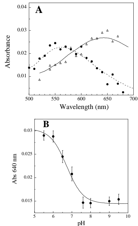
Figure 5. A. Absorption spectra of the final species formed at different pHs after the reaction of the E47A SOR mutant with O 2 •- (8 μM), generated by pulse radiolysis in the presence of 10 mM formate and 2 mM buffer. (Δ) pH 5.5, 4 ms after the pulse. (●) pH 8.5, 80 ms after the pulse. Tungsten lamp with a 345 nm cut-off filter, 2 cm path-length cuvette. The absorption spectrum in 2 cm path-length cuvette of the iridium chloride oxidized E47A SOR mutant (8 μM) is shown at pH 5.5 (solid line) and at pH 8.5 (dotted line). B. pH-dependence of the final absorbance at 640 nm measured after the reaction of the E47A SOR mutant from D. baarsii (100 μM) with O 2 •- (8 μM), under the same conditions. The titration curve fits the equation expected from a single protonation process, A_{640nm} = (A_{640max} + A_{640min} \times 10^{(pH-pK_a)}) / (1 + 10^{(pH-pK_a)}) . A pK a value of 6.7 ± 0.2 was determined.
