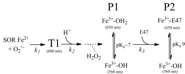
Scheme 1. Reaction mechanism of the SOR from D. baarsii with \text{O}_2^{\bullet -} deduced from pulse radiolysis studies. T1 is the only competent reaction intermediate observed by pulse radiolysis. P1 and P2 are reaction products formed after the release of \text{H}_2\text{O}_2 from the active site.
