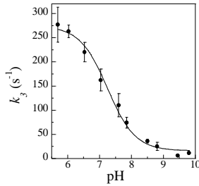
Figure 4. pH-dependence of the rate constant k_3 for the reaction of the wt SOR from D. baarsii (100 \mu\text{M} ) with \text{O}_2^{\bullet -} (8-12 \mu\text{M} ), generated by pulse radiolysis in the presence of 10 mM formate and 2 mM buffer. Tungsten lamp with a 345 nm cut-off filter. The titration curve fitted the equation expected from a single protonation process, k_3 = (k_{3\text{max}} + k_{3\text{min}} \times 10^{(\text{pH}-\text{pK}_a)}) / (1 + 10^{(\text{pH}-\text{pK}_a)}) . A \text{pK}_a value of 7.2 \pm 0.1 was determined.
