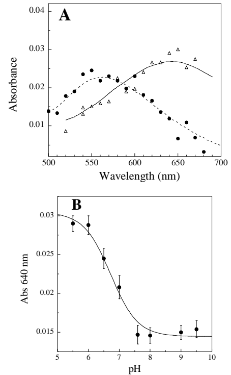
Figure 5. A. Absorption spectra of the final species formed at different pHs after the reaction of the E47A SOR mutant with \text{O}_2^{\bullet -} (8 \mu\text{M} ), generated by pulse radiolysis in the presence of 10 mM formate and 2 mM buffer. ( \Delta ) pH 5.5, 4 ms after the pulse. ( \bullet ) pH 8.5, 80 ms after the pulse. Tungsten lamp with a 345 nm cut-off filter, 2 cm path-length cuvette. The absorption spectrum in 2 cm path-length cuvette of the iridium chloride oxidized E47A SOR mutant (8 \mu\text{M} ) is shown at pH 5.5 (solid line) and at pH 8.5 (dotted line). B. pH-dependence of the final absorbance at 640 nm measured after the reaction of the E47A SOR mutant from D. baarsii (100 \mu\text{M} ) with \text{O}_2^{\bullet -} (8 \mu\text{M} ), under the same conditions. The titration curve fits the equation expected from a single protonation process, A_{640\text{nm}} = (A_{640\text{max}} + A_{640\text{min}} \times 10^{(\text{pH}-\text{pK}_a)}) / (1 + 10^{(\text{pH}-\text{pK}_a)}) . A \text{pK}_a value of 6.7 \pm 0.2 was determined.
