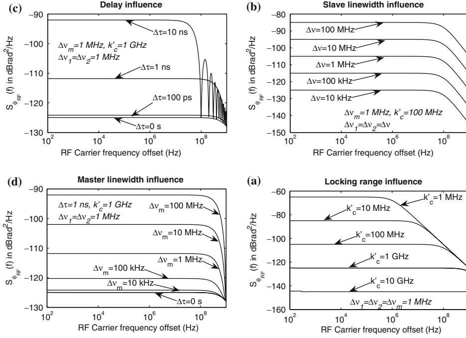
Fig. 2. RF phase power spectral density.
