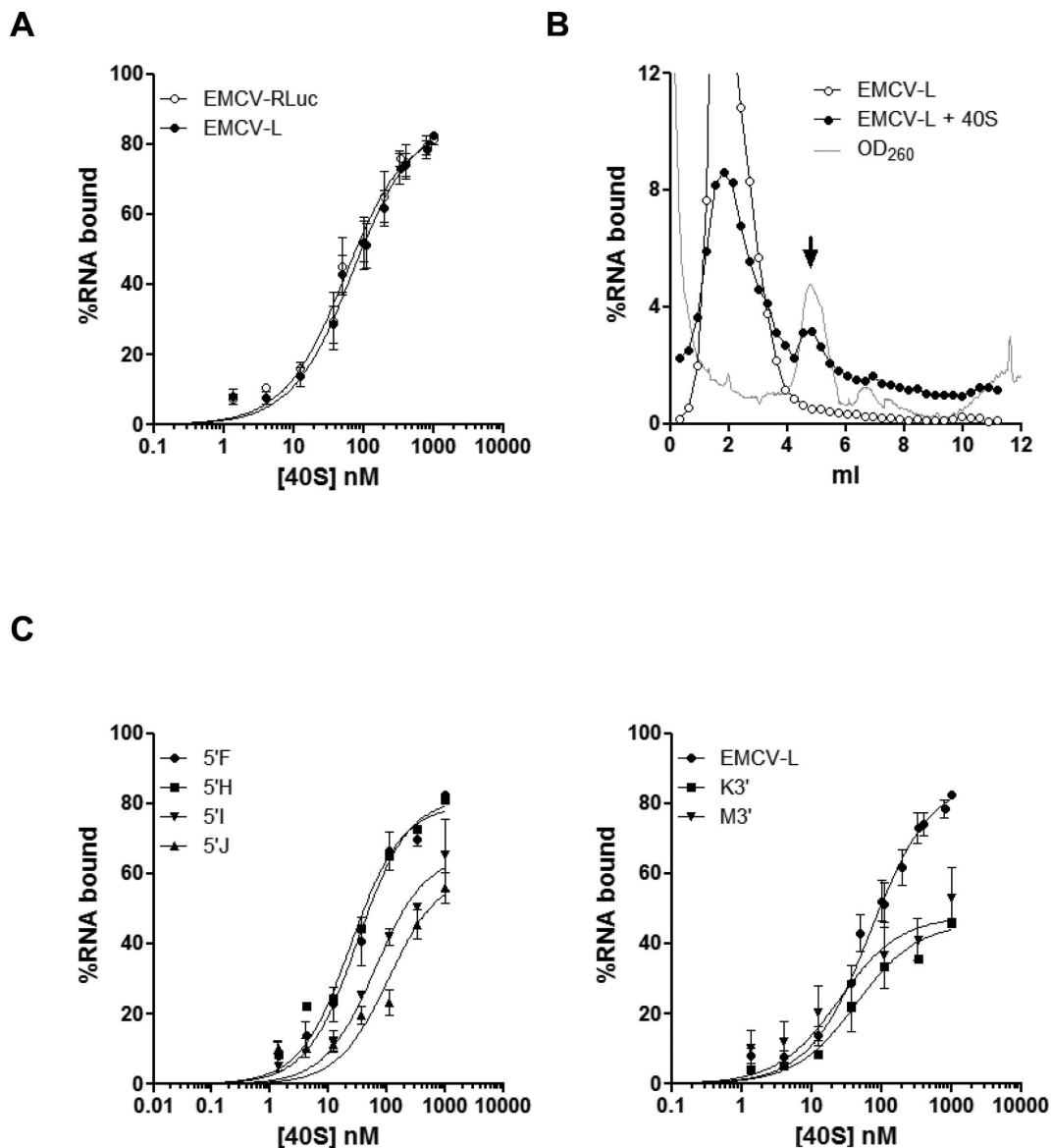
Figure 3. EMCV-L interaction with ribosomal 40S. (A) Binding curves of ^{32} P-labeled EMCV-RLuc ( \circ ) or EMCV-L ( \bullet ) to purified 40S ribosomal subunit. (B) Fractionation by 10–30% sucrose density gradient of EMCV-L in the absence ( \circ ) or presence ( \bullet ) of excess-purified 40S subunits. OD 260 profile in the presence of purified 40S is indicated in gray. (C) Binding curves of ^{32} P-labeled 5'- (left panel) or 3'-end (right panel) deletion mutants to purified 40S ribosomal subunit. 5'F: U 340 -A 905 ; 5'H: G 401 -C 905 ; 5'I: U 451 -C 905 ; 5'J: A 678 -C 905 ; K3': C 280 -C 785 ; M3': C 280 -A 840 . The results are the mean of at least three independent experiments \pm standard deviation.
