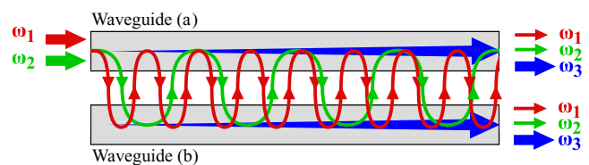
FIG. 1. (Color online) Schematic diagram of the principle of coupling-length phase-matching (CLPM). The two waveguides a and b are assumed to be identical. The pump beams (at frequency \omega_1 and \omega_2 in this example) are injected in waveguide a . The evanescent coupling between the two waveguides causes the power of the pump waves to oscillate between the two waveguides (schematically represented in this sketch by the two lines meandering between the two waveguides). Under the appropriate CLPM condition it is possible to arrange for the signal wave at frequency \omega_3 that is created by nonlinear optical interaction of the two pump waves to grow constructively with propagation length, in both waveguides. The qualitative depiction in this figure corresponds to the case of sum-frequency generation ( \omega_3 = \omega_1 + \omega_2 ) that will be presented later in Fig. 2.
