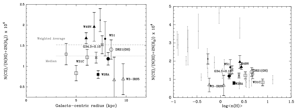
Fig. 10. Left : Ratio of the total C^+ column density to that of the total gas column measured by adding HI (from 21cm data) and H_2 (derived from CH and HF) as a function of Galacto-centric radius. The symbol size is proportional to the fraction of gas in molecular form ranging from \sim 0.1 to \sim 0.8 for the velocity intervals considered here, with each sight-line plotted with a different symbol. The weighted average ( 1.5 \times 10^{-4} ) is indicated with a dashed line and the median value ( 1.25 \times 10^{-4} ) with a dotted line. Right panel : comparison of the Herschel data (black symbols with source name) with the FUV absorption data from Parvathi et al. (2012) (gray dots with error bars). The gas-phase carbon abundance is plotted as a function of the logarithm of average gas density \log_{10}(\langle n(H) \rangle) = \log_{10}(N_{tot}(H)/L) .
