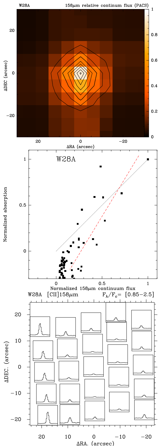
Fig. B.3. PACS data towards W28A at 158\ \mu\text{m} . For all maps, the offsets are given relative to the central position listed in Table 1. Top: Continuum emission at 158\ \mu\text{m} . Contour levels are 0.2, 0.3, 0.4 ... 0.9 relative to the maximum. Middle: Comparison of the integrated absorption measured in the HIFI map relative to the absorption at the map center, with the continuum flux measured in the PACS map relative to the map center. The dashed red line shows the linear regression line and the dotted black line a 1:1 relationship. Bottom: Map of the line to continuum emission/absorption in the 25 PACS spaxels. The vertical scale runs from 0.85 to 2.5. The data have not been corrected for the possible contamination in the OFF position.
