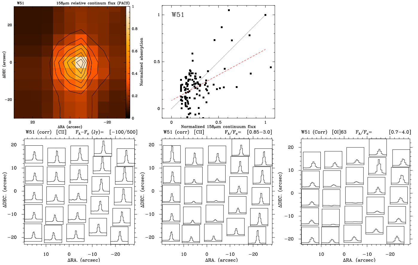
Fig. B.15. PACS data towards W51. For all maps, the offsets are given relative to the central position listed in Tab 1. Top left: Continuum emission at 158\mu\text{m} . Contour levels are drawn at 0.2, 0.3, 0.4 ... 0.9 relative to the maximum. Top right: Comparison of the integrated absorption measured in the HIFI map relative to the absorption at the map center, with the continuum flux measured in the PACS map relative to the map center. The dashed red line shows the linear regression line and the dotted black line a 1:1 relationship. Bottom left: [C II] emission in the 25 PACS spaxels. The continuum emission has been subtracted. The vertical scale runs from -100 to 500 Jy. Bottom middle: Map of the [C II] line to continuum emission/absorption in the 25 PACS spaxels. The vertical scale runs from 0.85 to 3. Bottom right: Map of the [O I] 63\mu\text{m} line to continuum emission/absorption in the 25 PACS spaxels. The vertical scale runs from 0.7 to 4.
