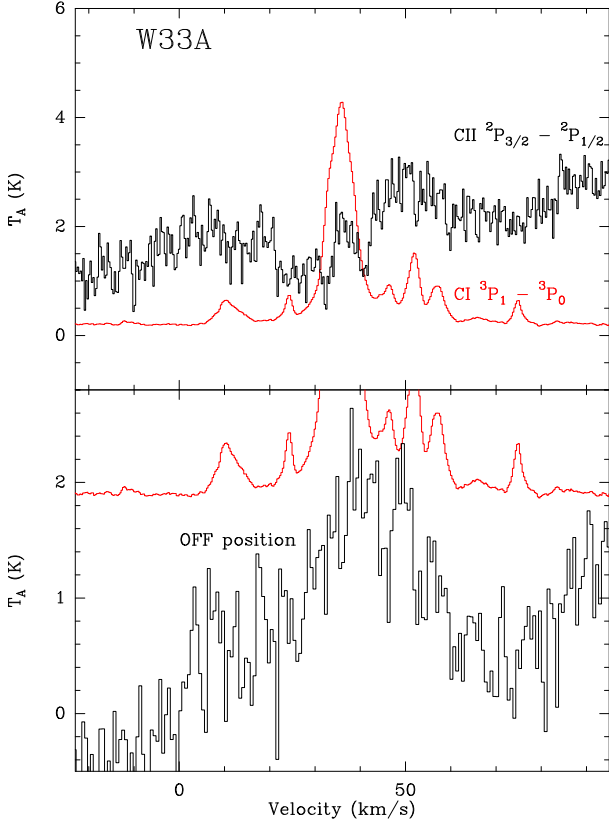
Fig. B.7. Top : Herschel/HIFI spectra towards W33A. The red line shows the [C I] ^3P_1 - ^3P_0 line at 492 \text{ GHz} and the black line the [C II] ^2P_{3/2} - ^2P_{1/2} line at 1.9 \text{ THz} . The horizontal axis is the LSR velocity in \text{km s}^{-1} , and the vertical axis the antenna temperature in Kelvins. The continuum level for [C II] corresponds to the SSB continuum levels. Bottom : zoom on the [C I] lines (red, as above), and average [C II] spectrum of the OFF positions (black). The continuum levels have been shifted for clarity in the bottom panel.
