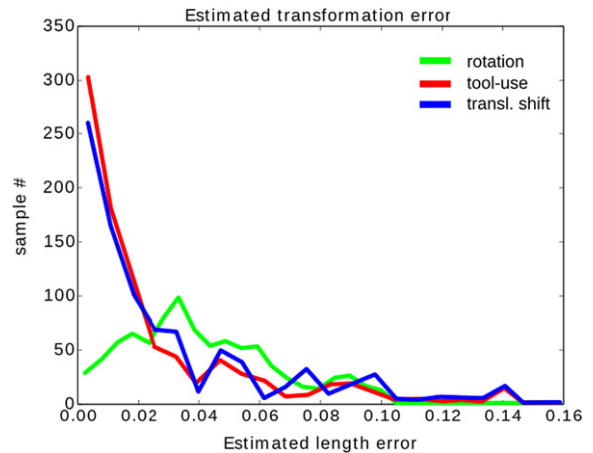
Fig. 9. Root mean square error computed from the position of the visual target and the estimated one for rotation (green), tool-use (red) and shift transformations (blue); resp. (a)–(c) in Fig. 8. The linear combination of gain-field neurons permit to reduce the error to a small range even for three different nonlinear transformations.
