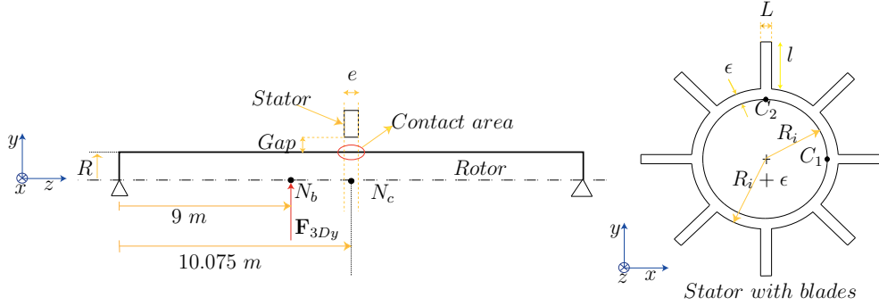
Figure 1: Dimensions of the rotor-stator system under study
