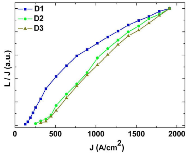
Figure 3. L/J versus J dependence for devices D1, D2 and D3.
