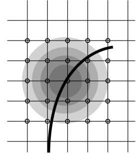
Fig. 3. Interpolation strategy.
