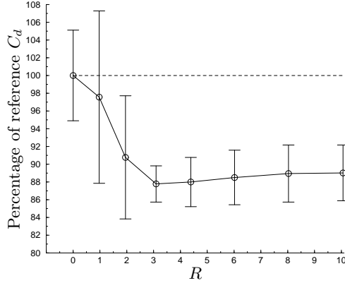
FIGURE 27. Effect of the resonant mode of the structure model on the drag, by varying the rigidity parameter from K_r = 3.7 \times 10^{-9} [ \text{kg m}^2 \text{s}^{-2} ] ( T_{flow}/T_{cilia} = 1 ) to K_r = 3.6 \times 10^{-7} ( T_{flow}/T_{cilia} = 10 ). The drag coefficient is plotted as a function of R = \omega_c \frac{T_{flow}}{2\pi} ; vertical bars indicate the amplitude of the temporal fluctuations of the drag coefficient.
