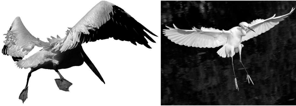
FIGURE 1. Raising of birds feathers, observed during landing phases. Left: snapshot of a pelican just before landing (thus gliding flight). Right: pop-up of feathers observed on the upper-side of the wings during the landing of an egret (courtesy of J R Compton, http://www.jrcompton.com/birds/ ).
