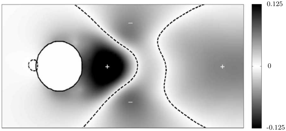
FIGURE 24. Contours of the non-dimensional scalar field \frac{\langle P^c \rangle - \langle P \rangle}{\rho \|\mathbf{U}_\infty\|^2} . The zero isocontours are shown in black dashed lines; white plus and minus signs refer to positive and negative zones.
