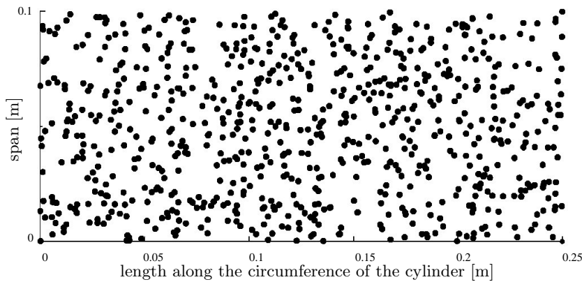
FIGURE 16. Visualisation of the density of hair (random organisation) on the unwrapped surface of a cylinder, for a packing density \phi = 0.006 , in a section of a hairy coating of length 0.25 [m] ( i.e. 40% of the perimeter of a cylinder of diameter 0.2 [m]) and span 0.1 [m]. 750 cilia of diameter 0.5 [mm] are represented by black circles in this control volume of 250 [cm 2 ].
