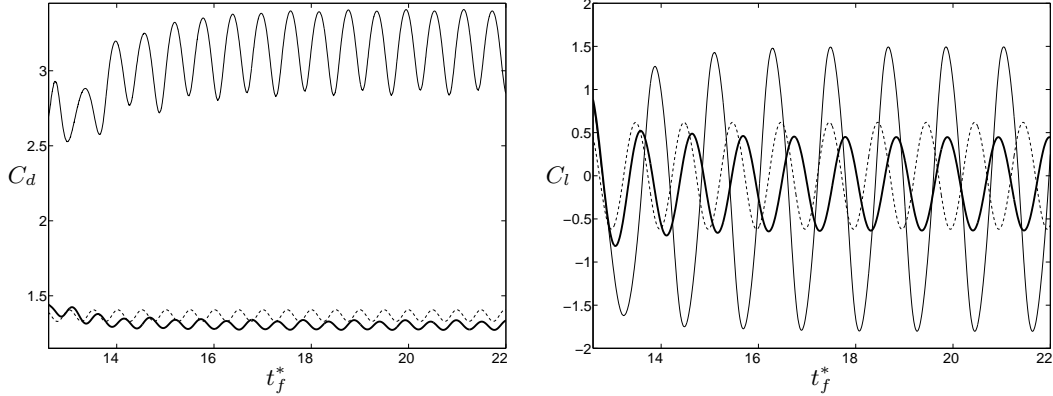
FIGURE 17. Aerodynamic coefficients corresponding to the static layers of figure 15. Left: Drag coefficient. Right: Lift coefficient. Dashed lines correspond to the configuration a) with smooth walls; thin solid lines correspond to the configuration b) with an orientation normal to the wall; bold lines correspond to the configuration c) with an orientation parallel to the flow.
