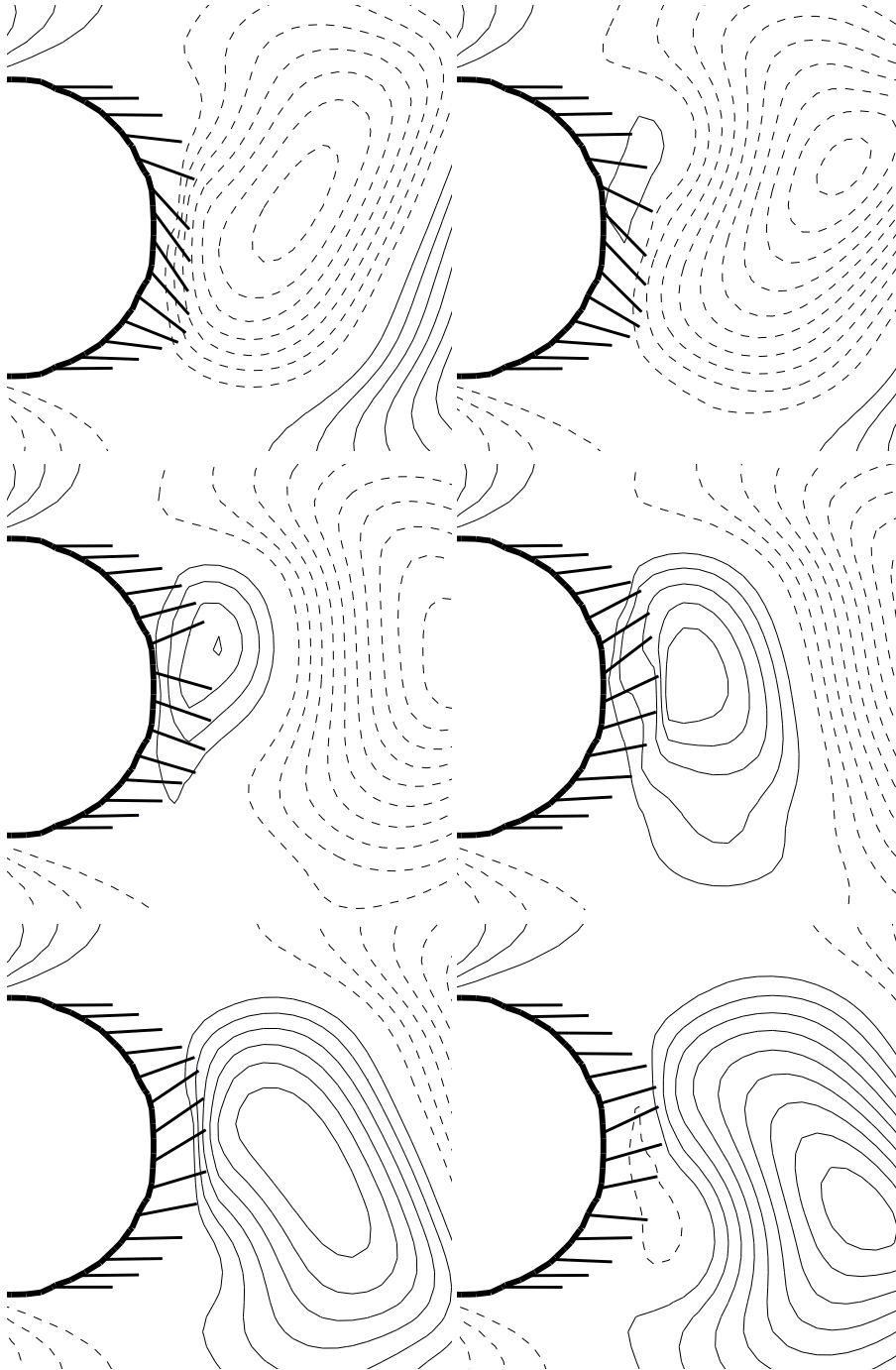
FIGURE 25. Motion of the reference cilia at the six time instants t_1 to t_6 shown in figure 22, arranged as in a comic strip (from left to right, and top to bottom). Snapshots of vertical velocity contours are displayed in the background (plain lines: positive, dashed lines: negative). The movement of the reference fibers is shown with the evolution of the vertical velocity in time in movie 2, available with the online version of the paper.
