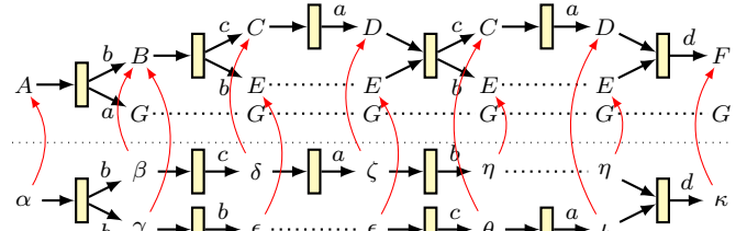
Figure 10: Embedding of a parallel run into the run from Figure 5.
