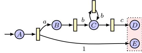
Figure 11: A Petri automaton for 1 \cap a \cdot b^+ \cdot c .
