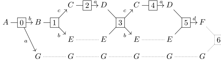
Figure 6: An accepting run in the automaton from Figure 5
