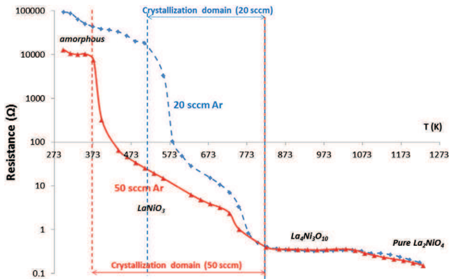
Fig. 7. Resistance of as deposited coatings of \text{La}_2\text{NiO}_4 composition deposited with 20 sccm ( \text{La/Ni} = 1.94 ) or 50 sccm Ar ( \text{La/Ni} = 2.04 ) as a function of the annealing temperature.
