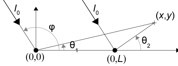
Figure 4: Double diffraction. The source is at infinite with incidence \varphi , the receiver at (x, y) and the diffracting points at (0, 0) and (0, L) . The emission angle is \theta .
