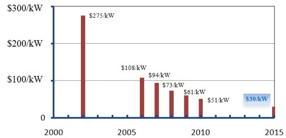
Fig.3 Modeled cost of an 80-kWPEM fuel cell system from [42]
