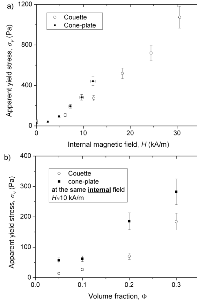
Fig. 3. Comparison of the experimental dependencies of the apparent yield stress on the internal magnetic field (a), and on the particle volume fraction (b), obtained for the cone-plate and the cylindrical Couette geometries. For the results presented in (a), the particle volume fraction is \Phi=0.3 . For the results presented in (b), the internal magnetic field is adjusted to H \approx 10 kA/m. The internal magnetic field is calculated in Appendix B as a function of the MR sample shape, its magnetic properties and the external field.
