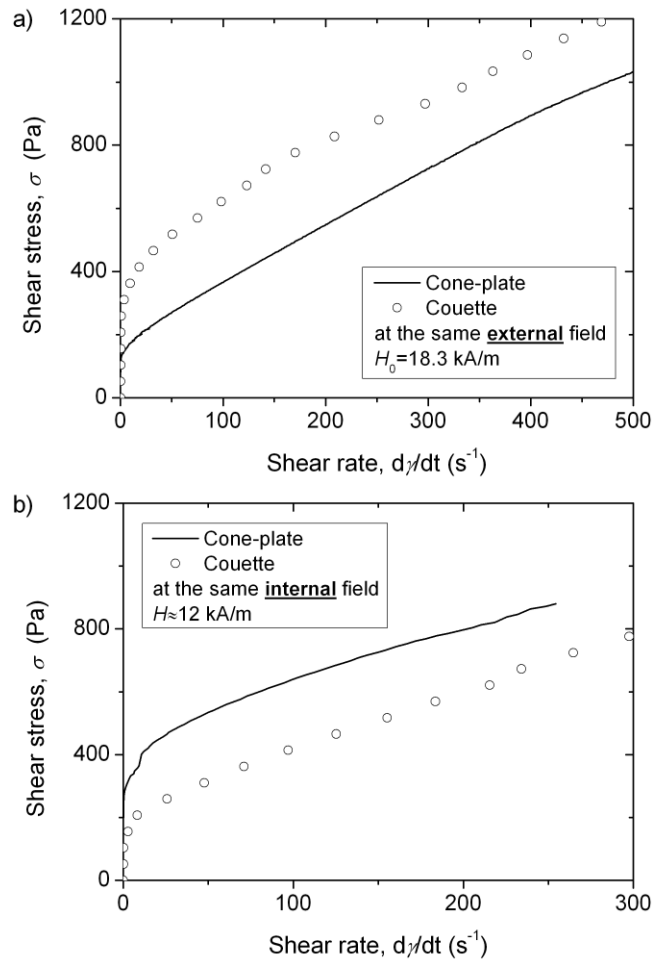
Fig.2. Comparison between the MR fluid flow curves measured in the cone-plate and the cylindrical Couette geometries at the same external magnetic field H_0 = 18.3 kA/m (a), and at the same internal magnetic field H \approx 12 kA/m (b). For both figures, the particle volume fraction is \Phi = 0.3
