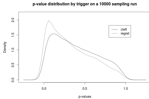
Fig. 1.2 p-value distribution
