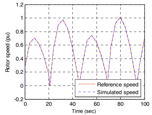
Fig. 9. 5-Phase PMSG speed and its reference in faulty mode.
