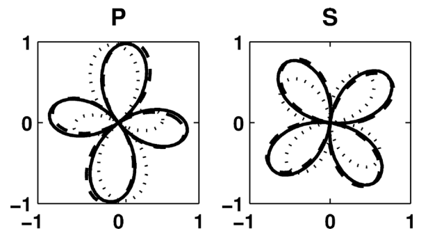
FIG. 4. Two-dimensional P- and S-wave radiation patterns of the source projected in the direction of M6 (solid), M7 (dashed), M8 (dotted) relative to the epicenter.
