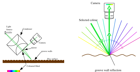
Fig. 1. Device Schematics
