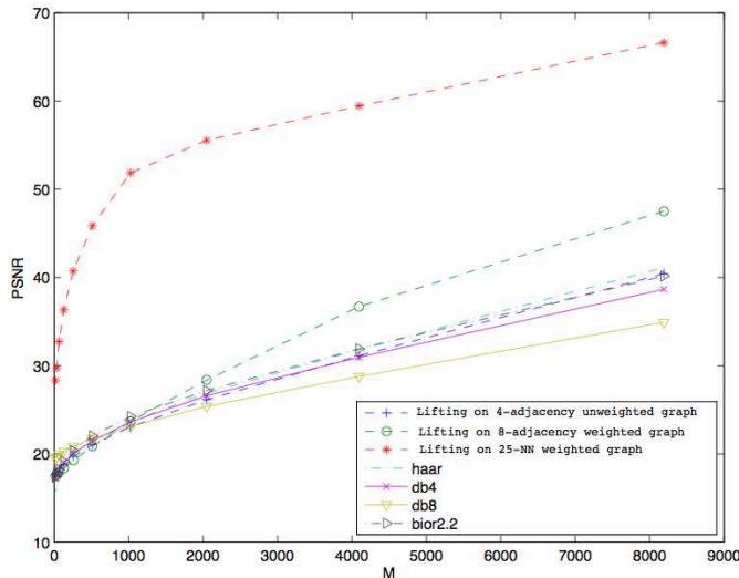
Fig. 2. M-term nonlinear approximation errors for “Barbara”. Transforms : lifting on graphs (4 et 8 adjacency, nearest neighbors), Haar, Daubechies 4, Daubechies 8, CDF(2,2).
