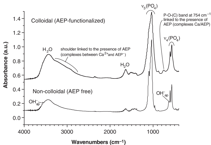
Figure 2. FTIR spectrum for colloidal biomimetic apatite (AEP-functionalized, prepared at 100^\circ\text{C} and pH 9.5), and for a non-colloidal (AEP-free) counterpart. FTIR: Fourier-transform infrared; AEP: 2-aminoethylphosphoric acid.
