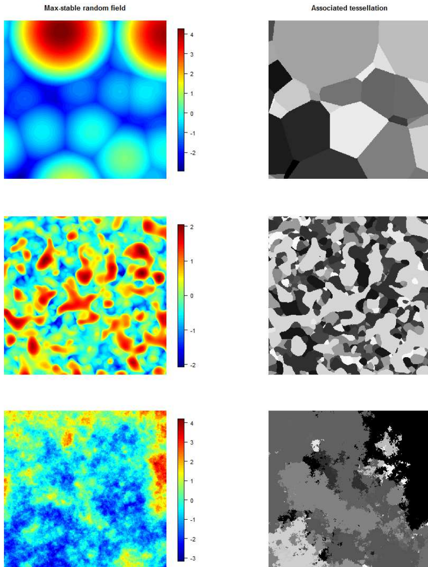
Figure 1: Realizations of a max-stable random field on \mathcal{X} = [-5, 5]^2 (left column) and of the associated tessellation (right column) for various models. Top: the Smith model with Gaussian shape function (Example 8). Middle: the extremal Gaussian model with Gaussian correlation \rho(h) = \exp(-\|h\|^2/2) (Example 9). Bottom: the Brown–Resnick model with variogram \gamma(h) = 2\|h\| (Example 10). To obtain a better contrast, max-stable random fields are plotted with Gumbel margins.
