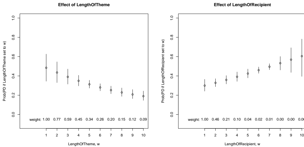
Figure 1: Representing the effects of the integer valued information variables.
