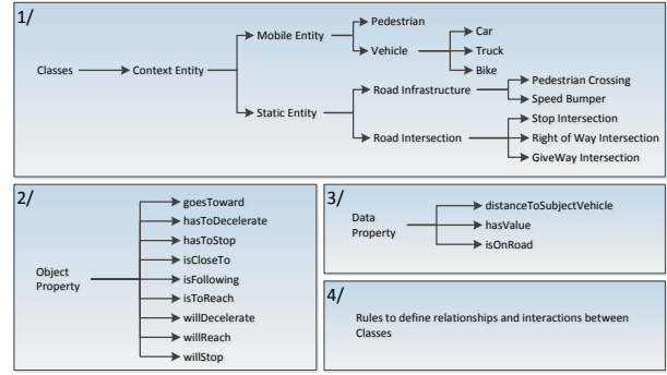
Fig. 3: Classes, objects and data properties defined in the ontology.
